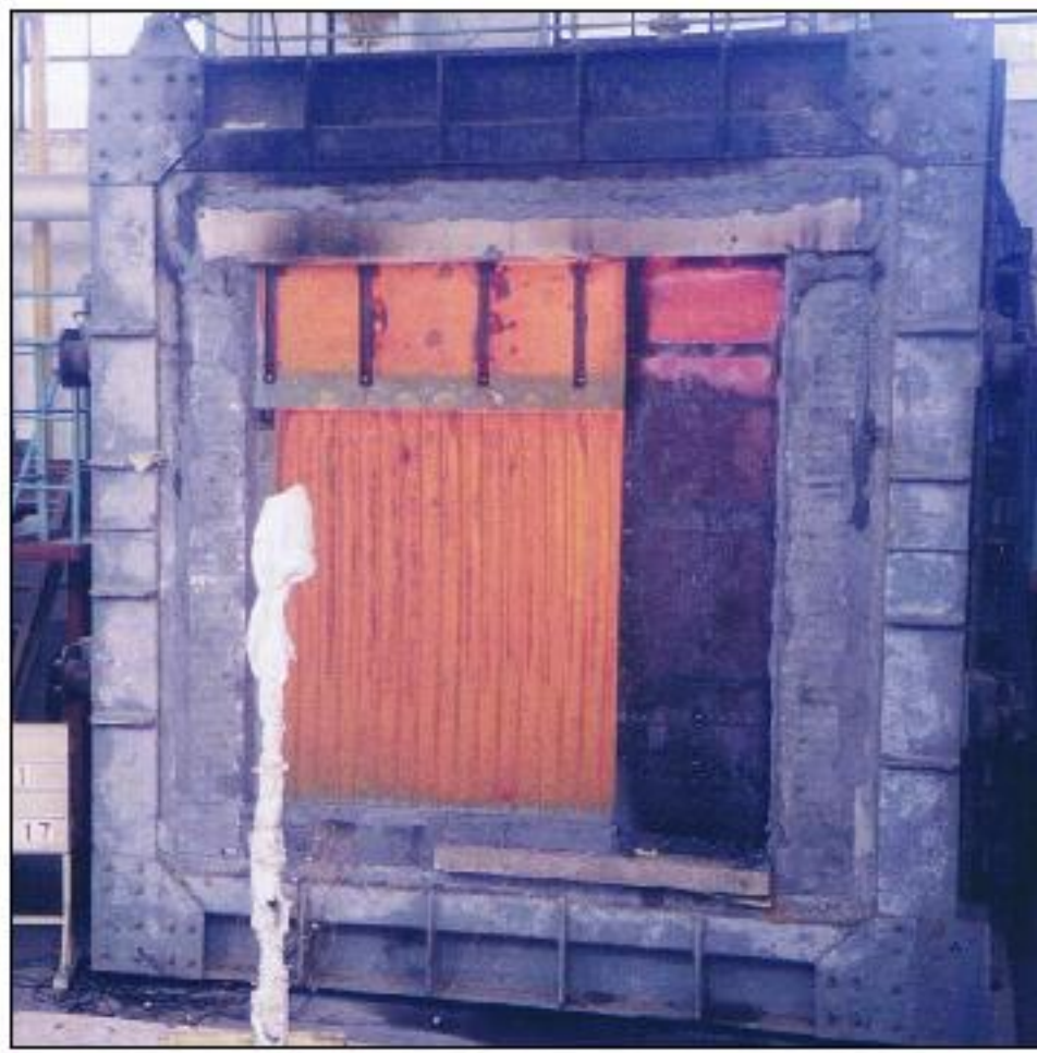
Lateral Sliding
